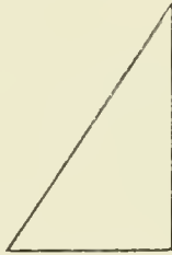
A TRIANGLE HAVING A RIGHT ANGLE AND THREE UNEQUAL SIDES.
